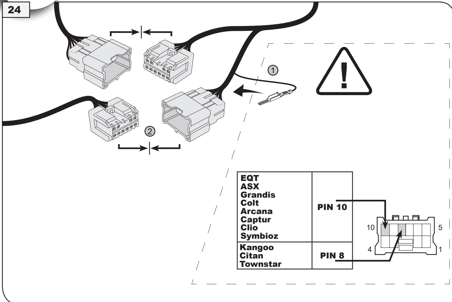
Auto Stecker car socket
